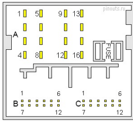
40 (16+12+12) pin QuadLock Fakra Head Unit / Car Stereo connector at the car stereo
