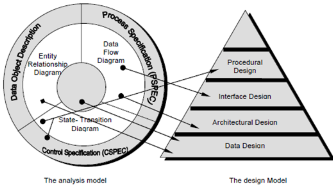
Figure 1. Translating the analysis model into a software design
