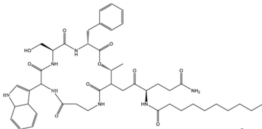
Ophiotine (45)
